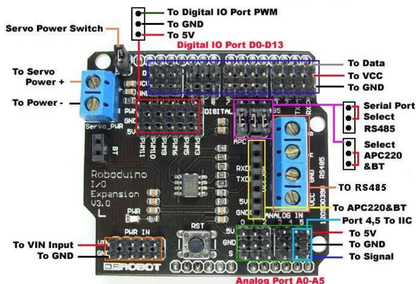
-Servo Power Switch- If uses internal 5V power apply the jumper, otherwise uses external Servo power.
